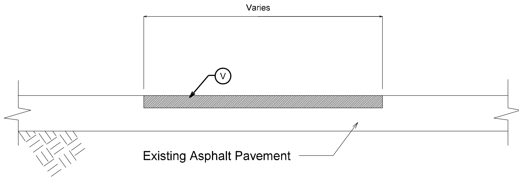
Asphalt Pavement Repair Typical Section
